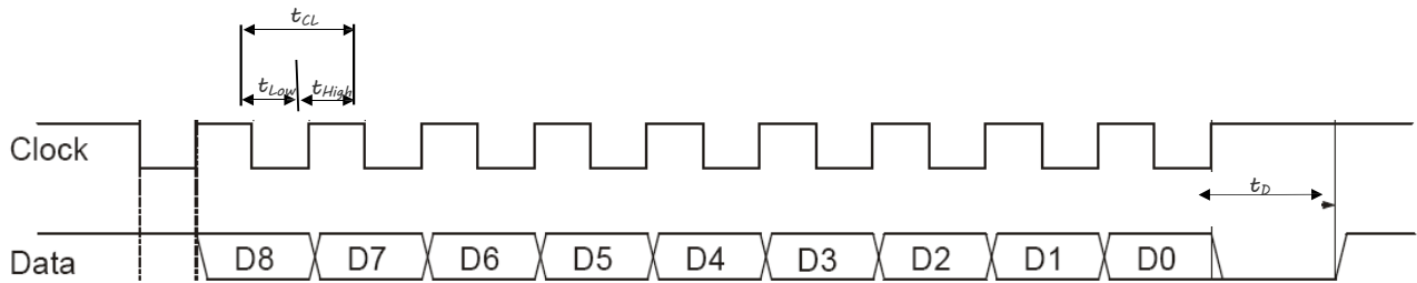
Figure 3: SSI timing diagram
