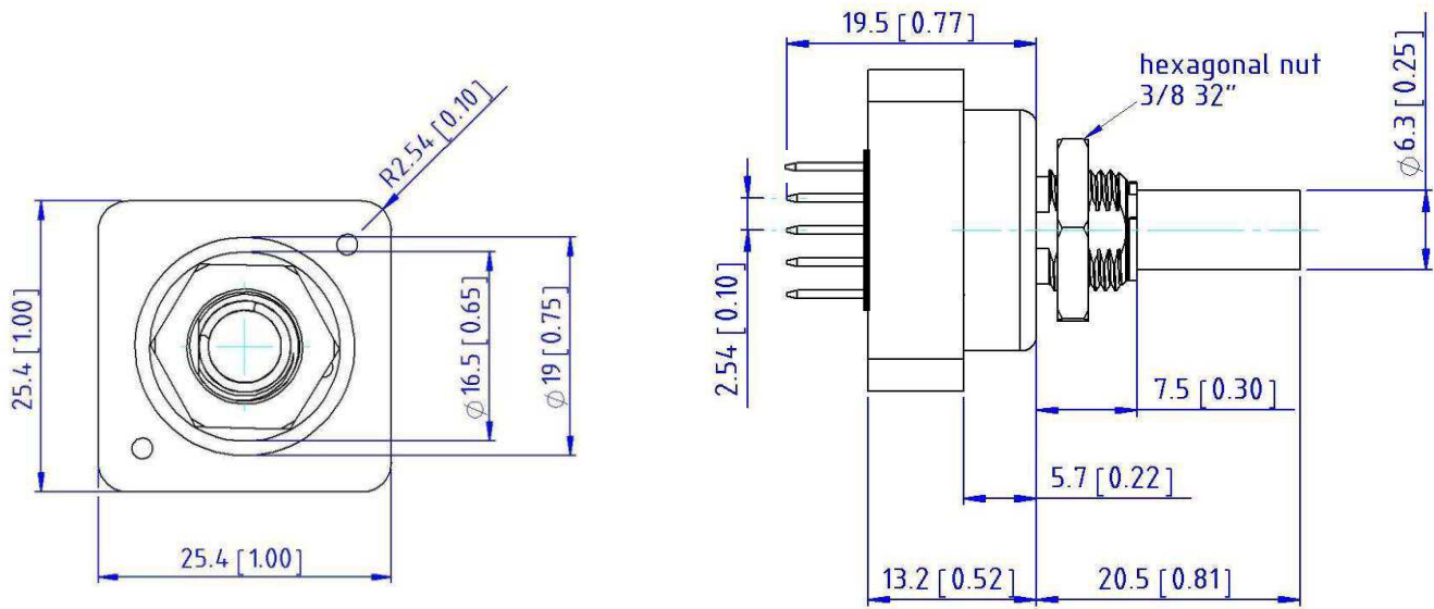
Figure 1: Dimensions of the ED-17-BB-512-S-P (top and side view)
